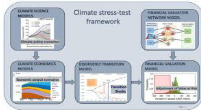
https://www.researchgate.net/figure/Diagram-illustrating-the-information-flow-in-the-climate-stress-test-framework_fig2_340815563
